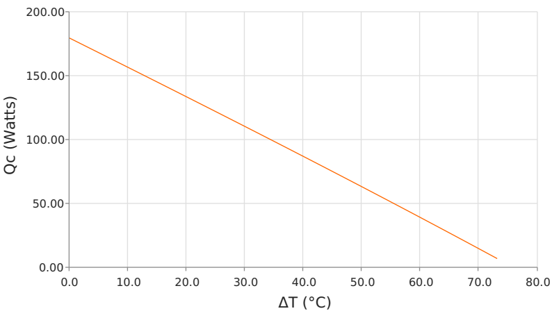
Heat Pumped at Cold Side ( Q_c ) T_{hot} = 50\text{ }^{\circ}\text{C} | operating = 9.4 Amps
