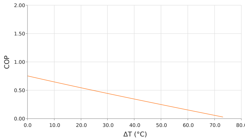
Coefficient of Performance (COP = Q_c/P_{in} ) T_{hot} = 50\text{ }^{\circ}\text{C} | operating = 9.4 Amps
