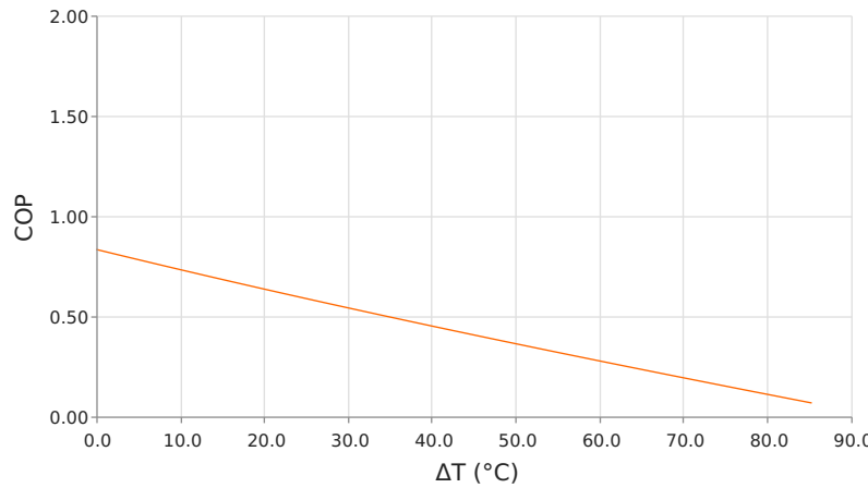
Coefficient of Performance (COP = Q_c/P_{in} ) T_{hot} = 85^\circ\text{C} | operating = 6.5 Amps
