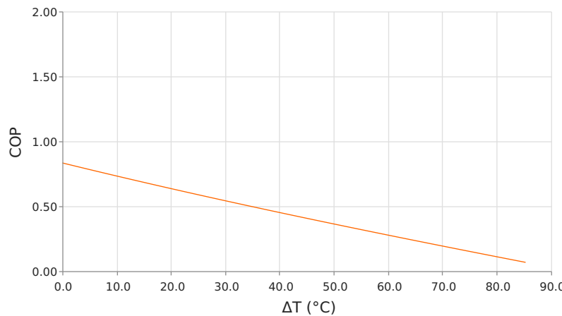
Coefficient of Performance (COP = Q_c/P_{in} ) T_{hot} = 85^\circ\text{C} | operating = 11.8 Amps
