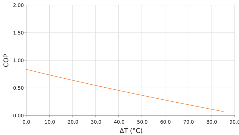
Coefficient of Performance (COP = Q_c/P_{in} ) T_{hot} = 85\text{ }^{\circ}\text{C} | operating = 11.5 Amps
