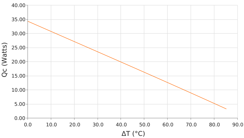
Heat Pumped at Cold Side ( Q_c ) T_{hot} = 85\text{ }^{\circ}\text{C} | operating = 11.5 Amps
