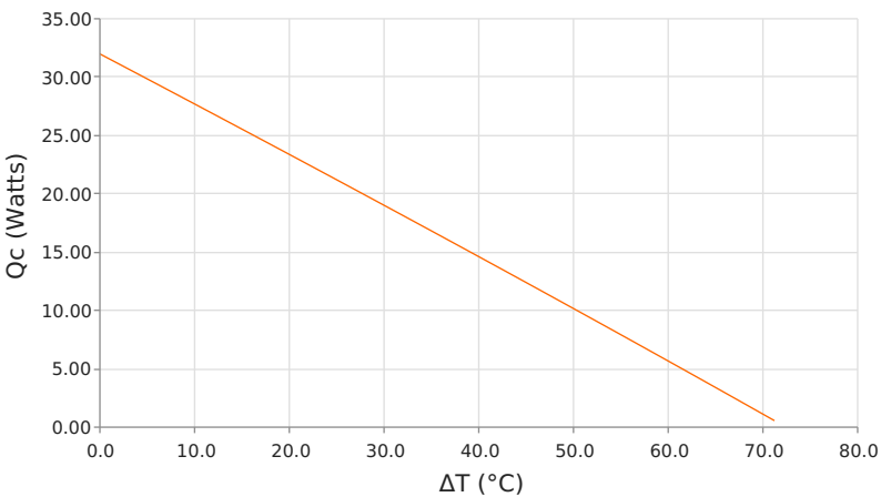
Heat Pumped at Cold Side ( Q_c ) T_{hot} = 35^\circ C | operating = 3.4 Amps
