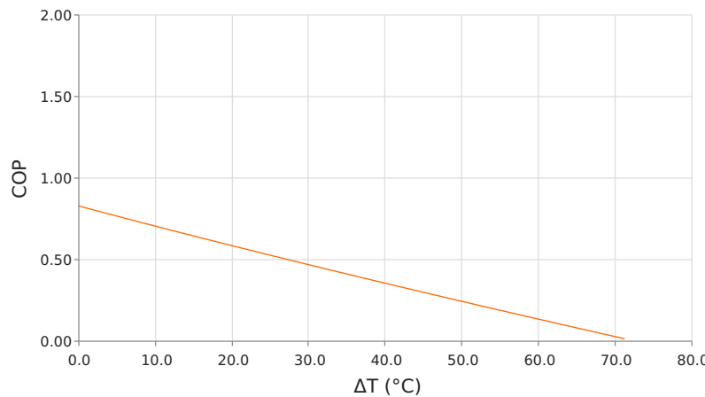
Coefficient of Performance ( COP = Q_c/P_{in} ) T_{hot} = 35^\circ C | operating = 3.4 Amps
