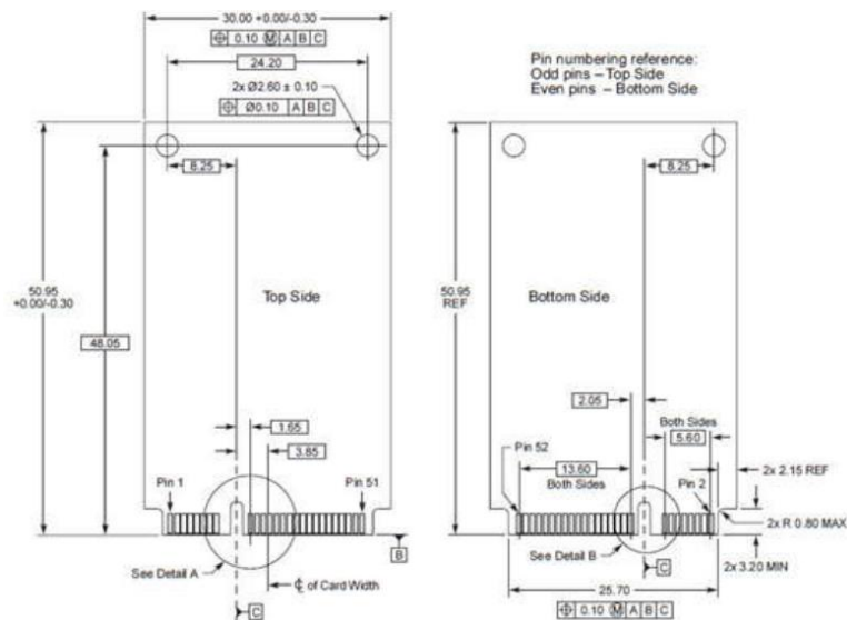
Figure 3: EVIA Mini PCIe USB Dimensions in mm
