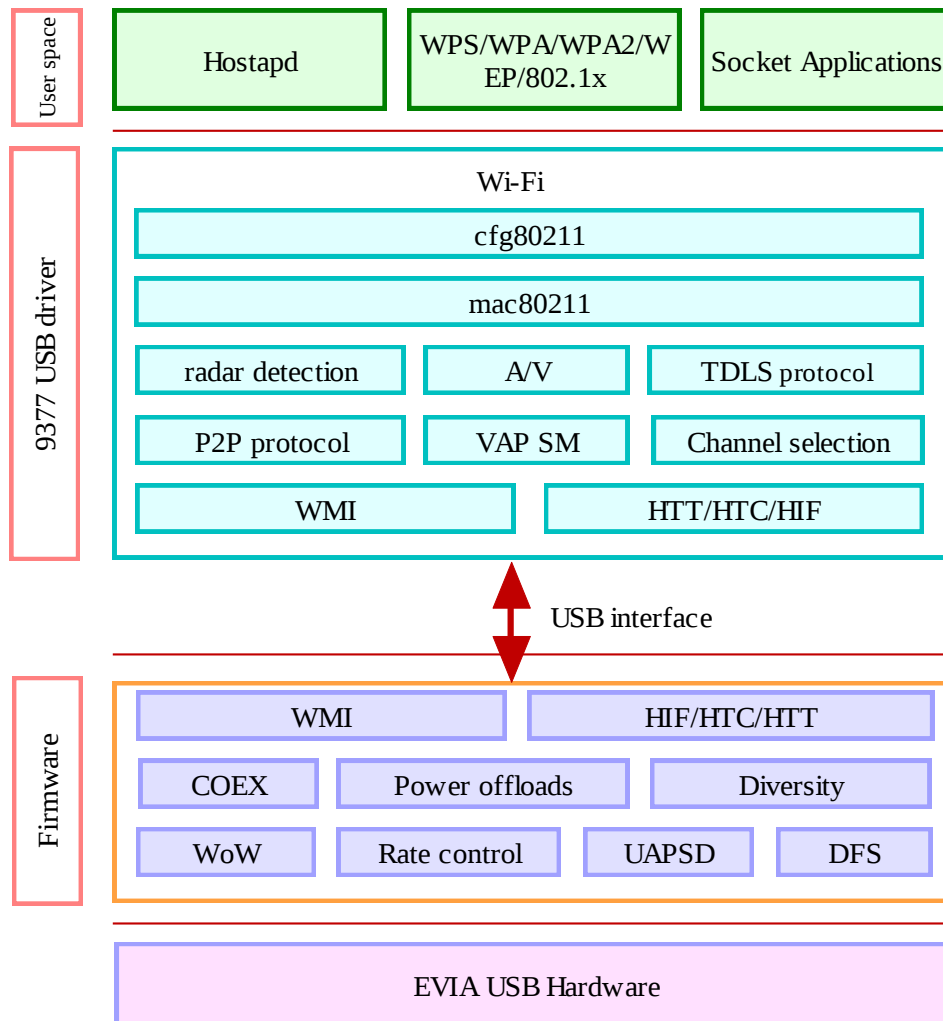
Figure 2: EVIA Software Architecture
