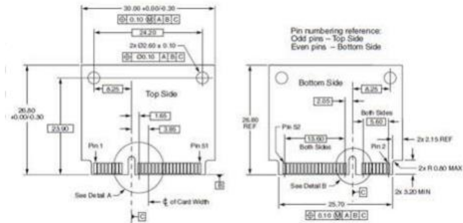
Figure 4: EVIA Half Mini PCIe USB Dimensions in mm
