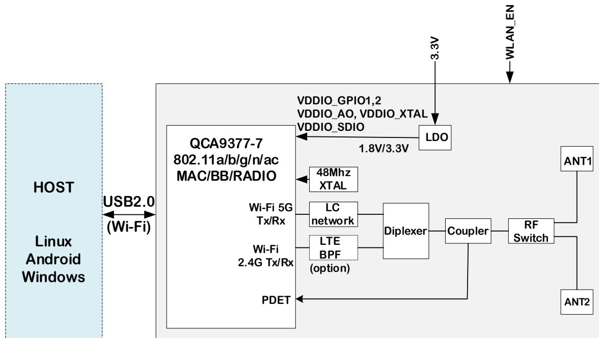
Figure 1: EVIA mPCIe USB card Block Diagram
