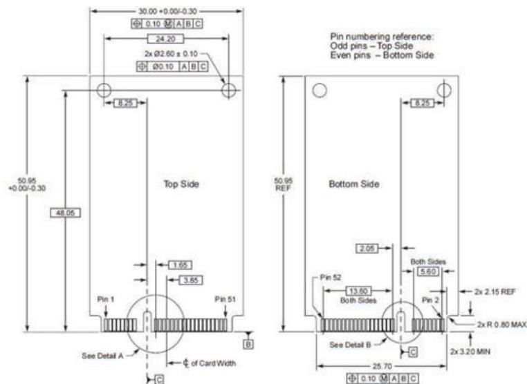
Figure 3: EVIA Mini PCIe Dimensions in mm
