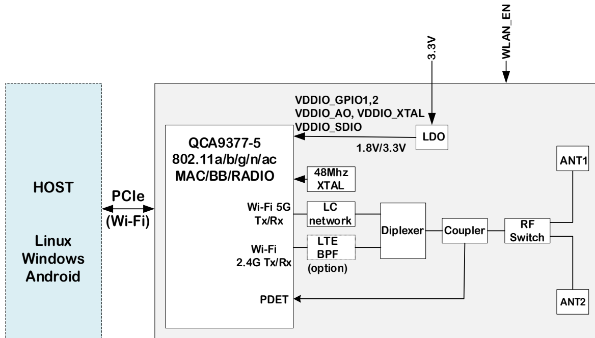
Figure 1: EVIA Mini PCIe card Block Diagram
