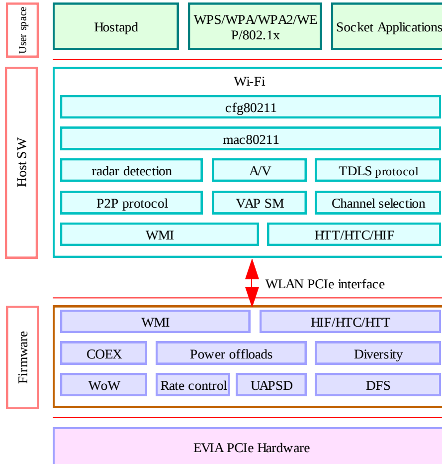
Figure 2: EVIA mPCIe Card Software Architecture
