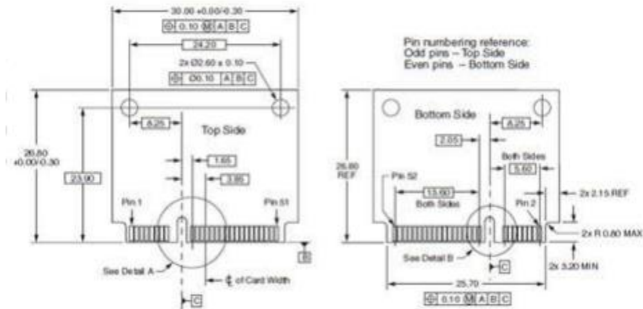
Figure 4: EVIA Half Mini PCIe Dimensions in mm
