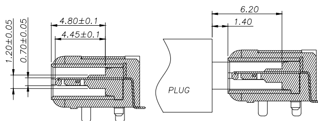
AFTER MATING
