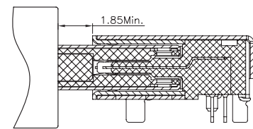
MATING CONDITION
