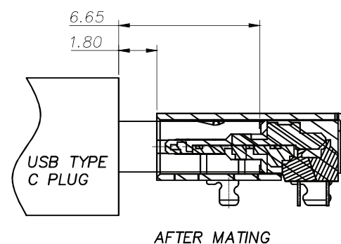
AFTER MATING
