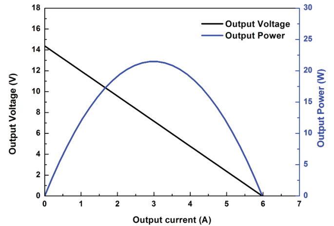
Output Voltage/Power Vs. Output Current (Th=300°C, Tc=30°C)
