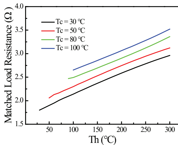
Matched Load Resistance Vs. Th
