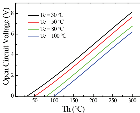
Open Circuit Voltage Vs. Th
