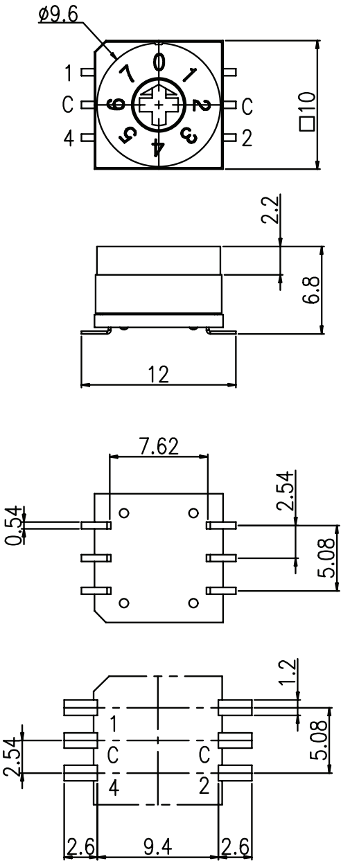
Recommended PCB Layout Top View
