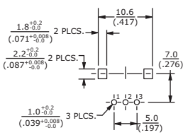
Recommended PCB Layout Top View
