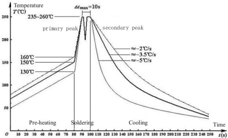
Double-wave Soldering Curve
