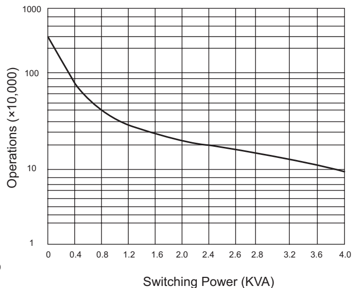
Life Curve
