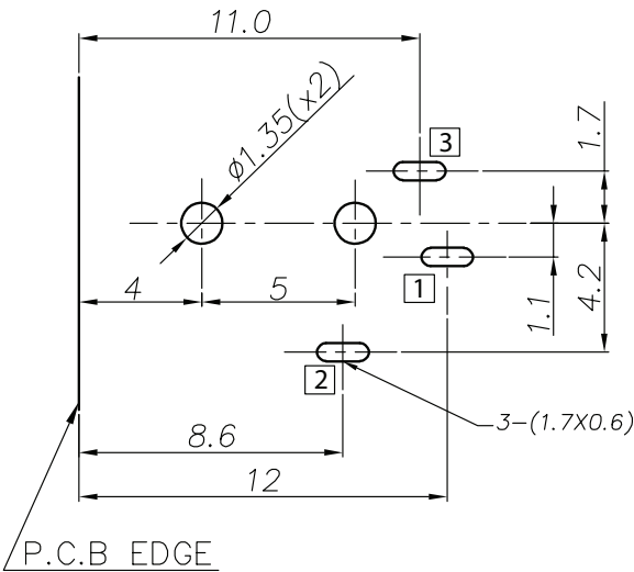
P.C.B. EDGE Recommended PCB Layout Top View
