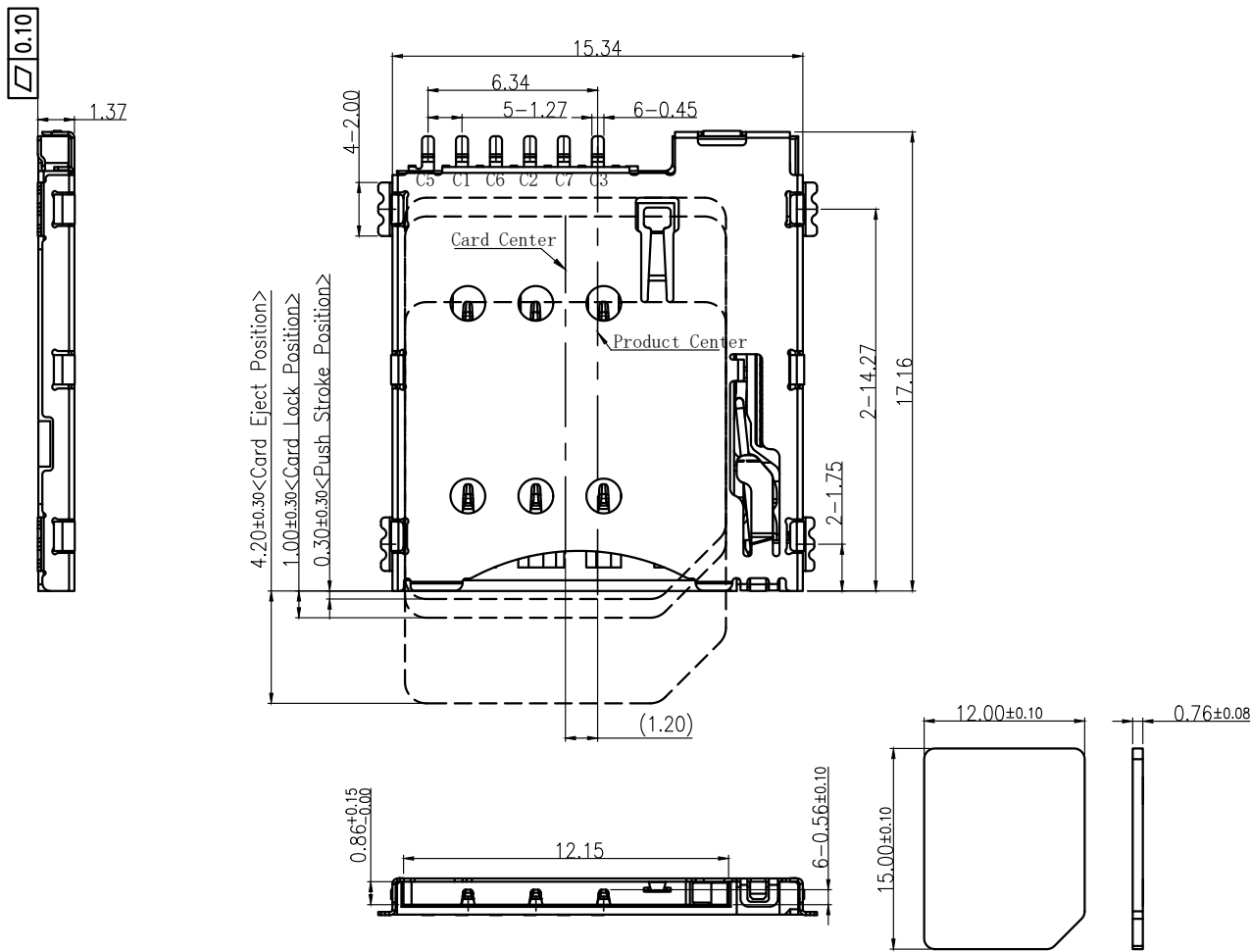
Micro SIM
