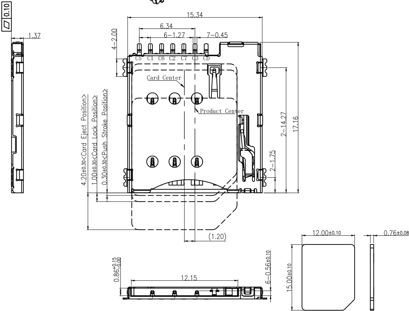
Micro SIM
