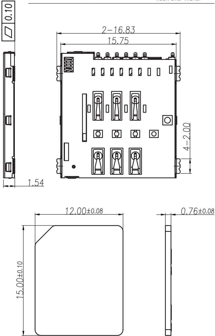
MICRO SIM
