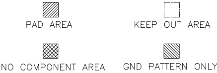
Recommended PCB Layout Top View
