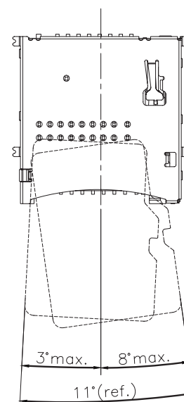
Card Insertion Guide Angle
