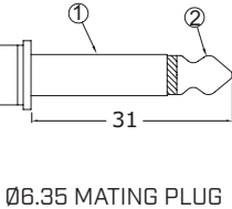
Ø6.35 MATING PLUG
