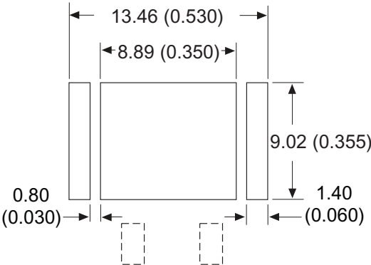
Recommended Solder Mask Opening Top View
