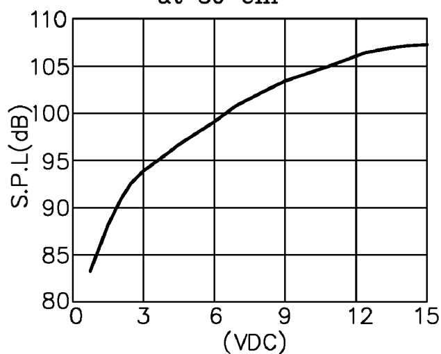
Voltage vs. Sound Pressure Level at 30 cm
