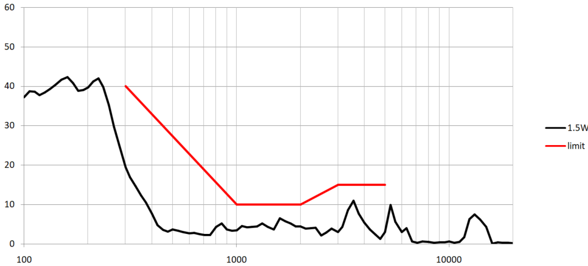
Total Harmonic Distortion Curve
