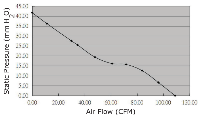
CFM-9238BF-280-585
