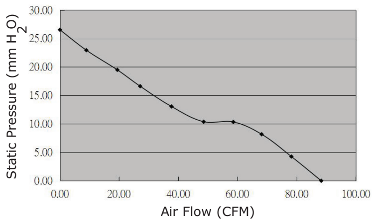
CFM-9238BF-295-628
