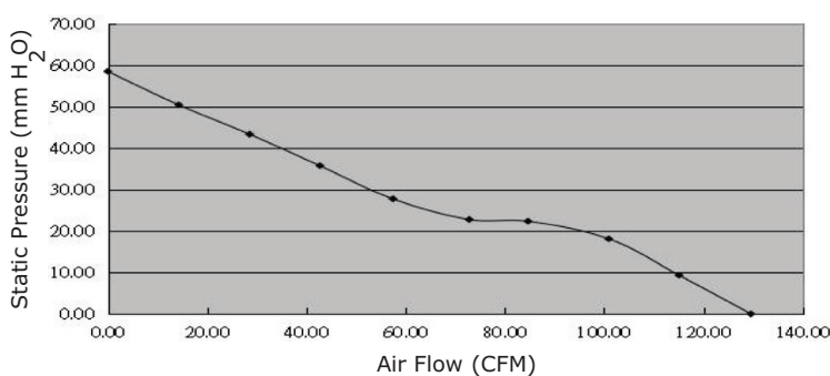
CFM-9238BF-295-628
