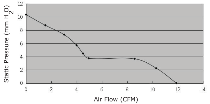
CFM-4020CF-195-342
