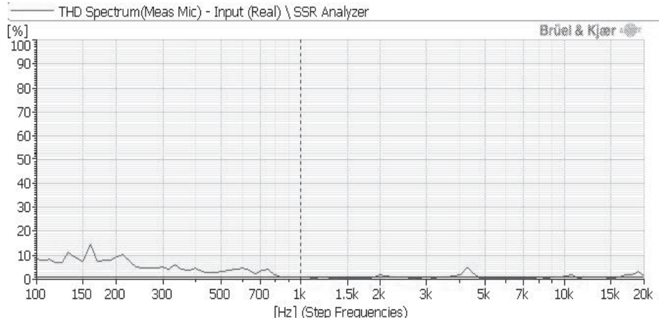
Total Harmonic Distortion Curve
