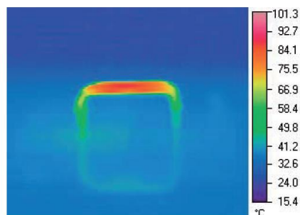
OAR1-R005 at 1W Hot spot: 87°C Solder joint: 45°C
