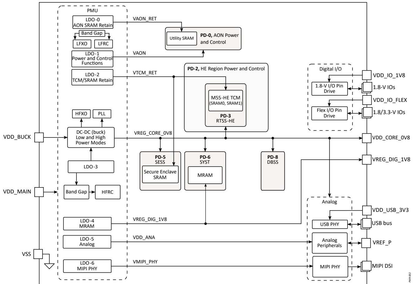
Figure 3-3 Device Voltage Distribution
