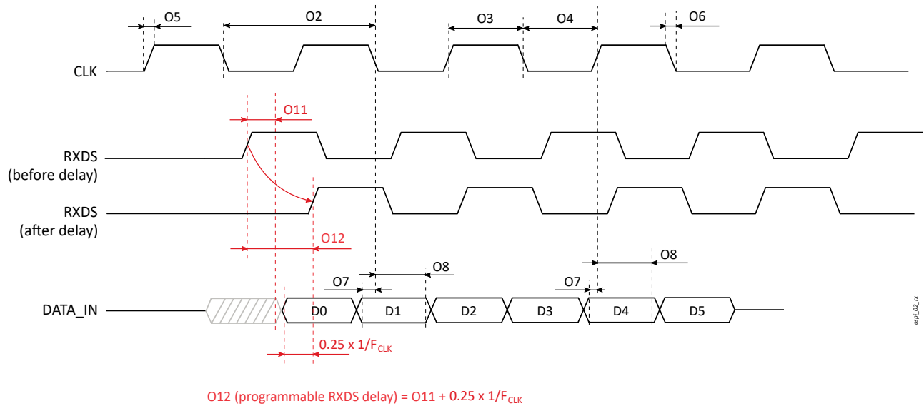
Figure 5-15 OSPI Timing Diagram - DDR Mode (Receive)
