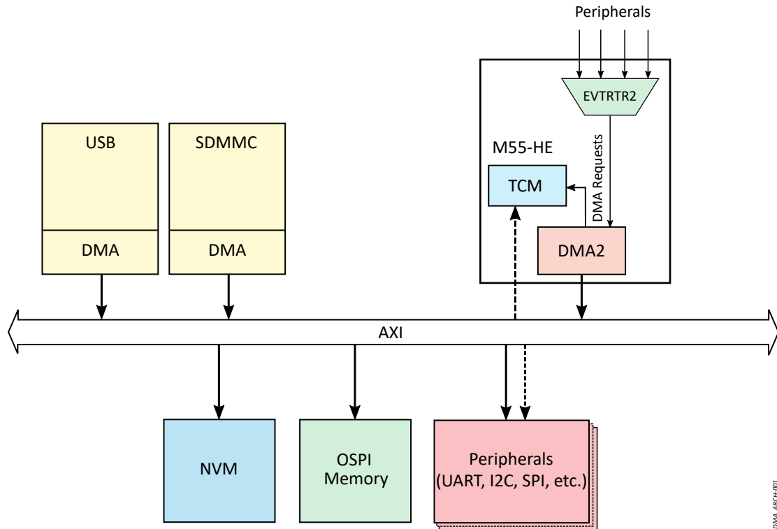
Figure 3-10 DMA Architecture
