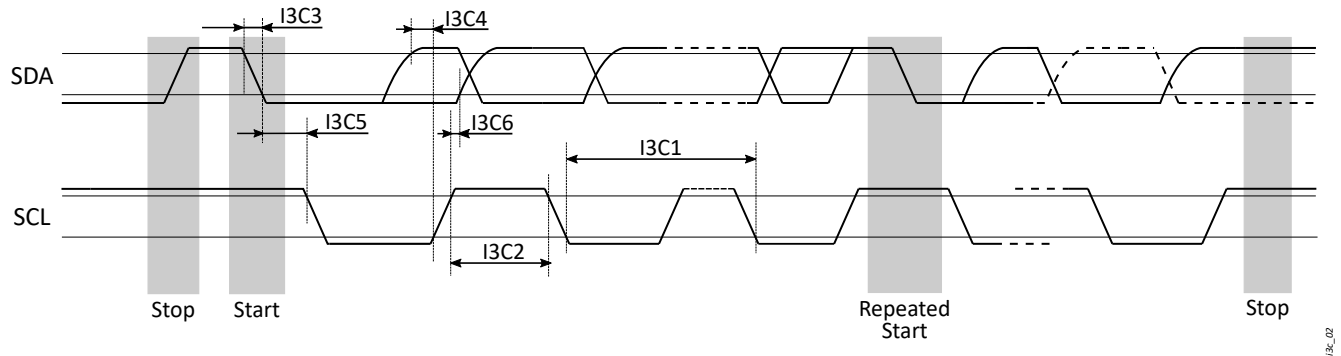
Figure 5-8 I3C Push-Pull Timing Diagram
