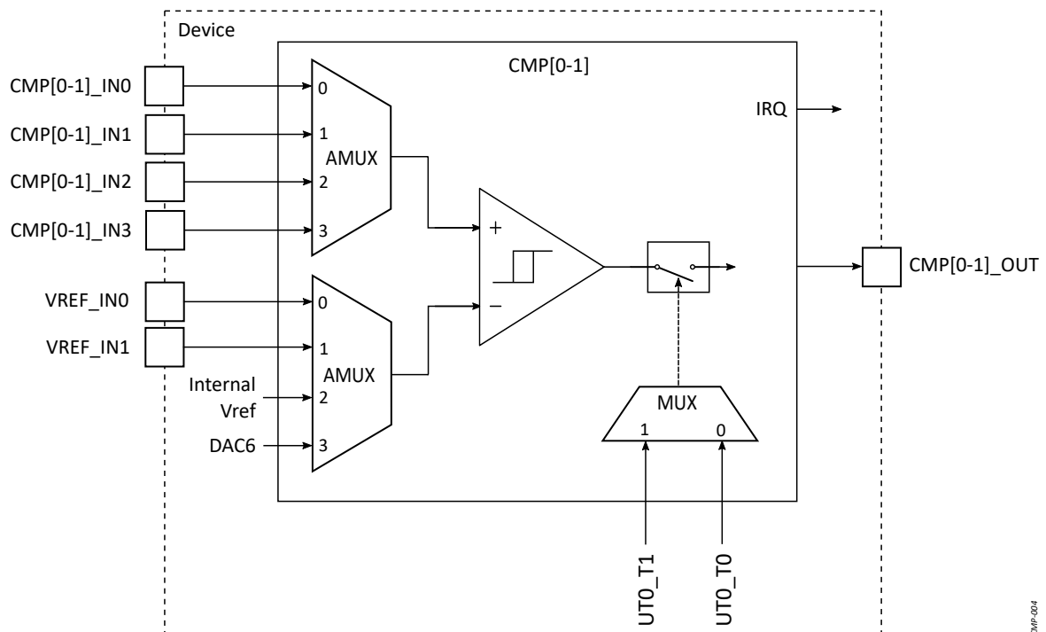
Figure 3-11 CMP Overview
