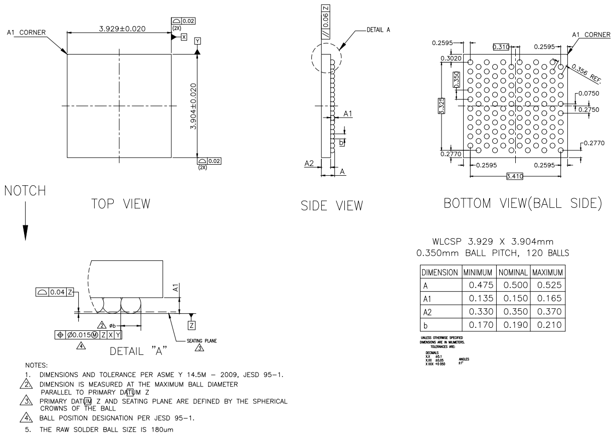
Figure 6-3 WLCSP120 Package Outline (1)
