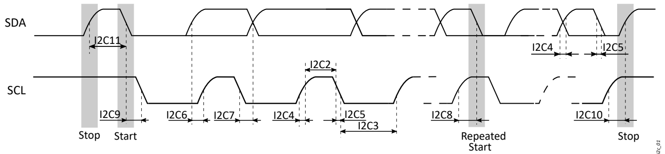
Figure 5-4 I2C Timing Diagram
