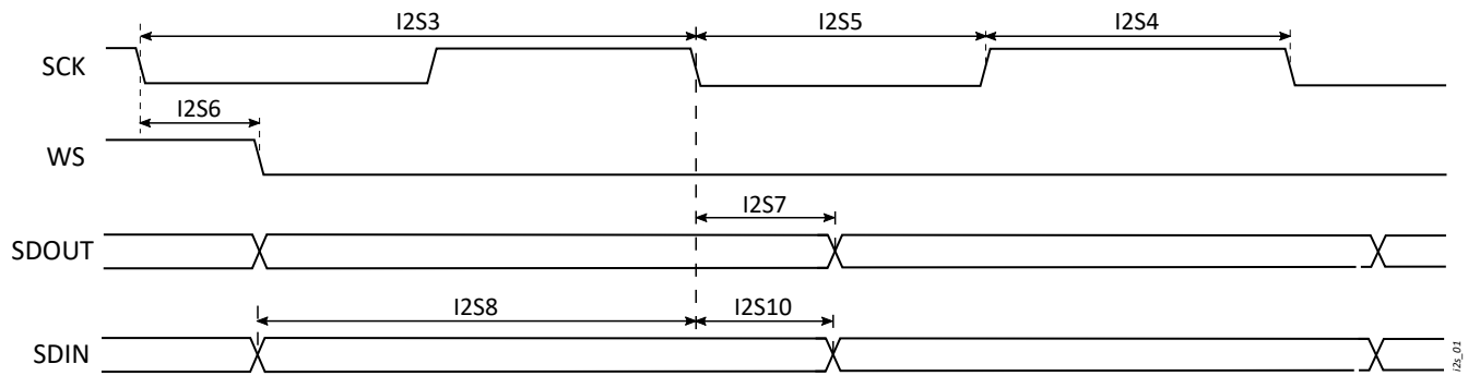
Figure 5-5 I2S Master Mode Timing Diagram
