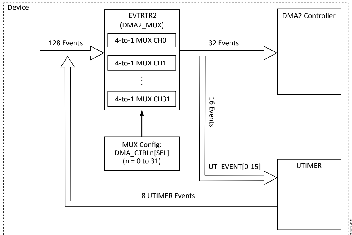
Figure 3-9 EVTRTR Overview
