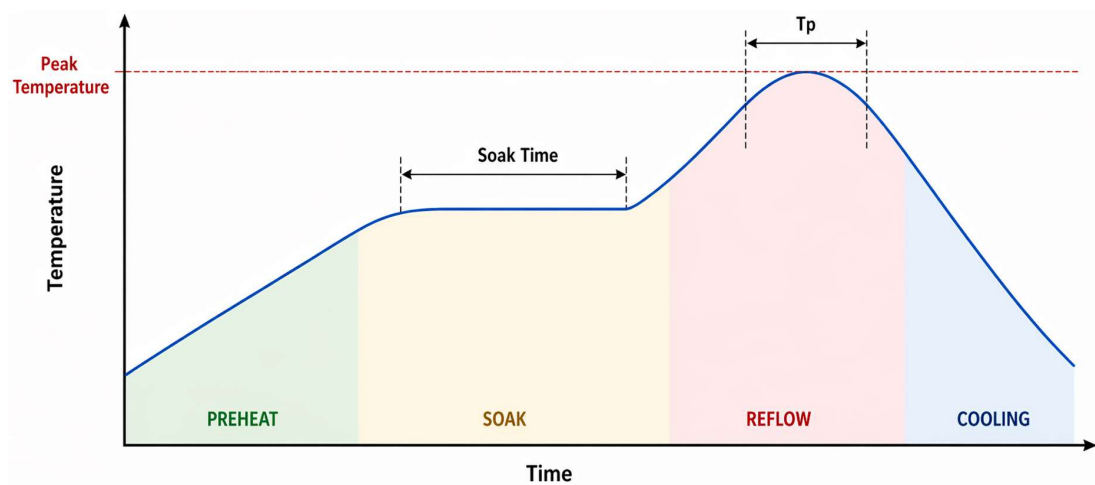
Figure 6-5 WLCSP120 Solder Reflow Profile
