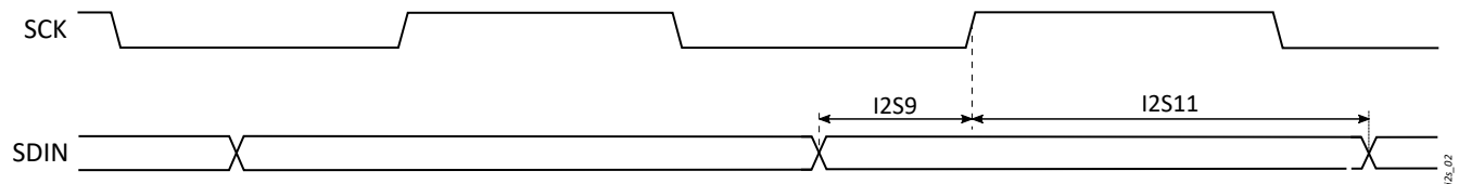
Figure 5-6 I2S Slave Mode Timing Diagram
