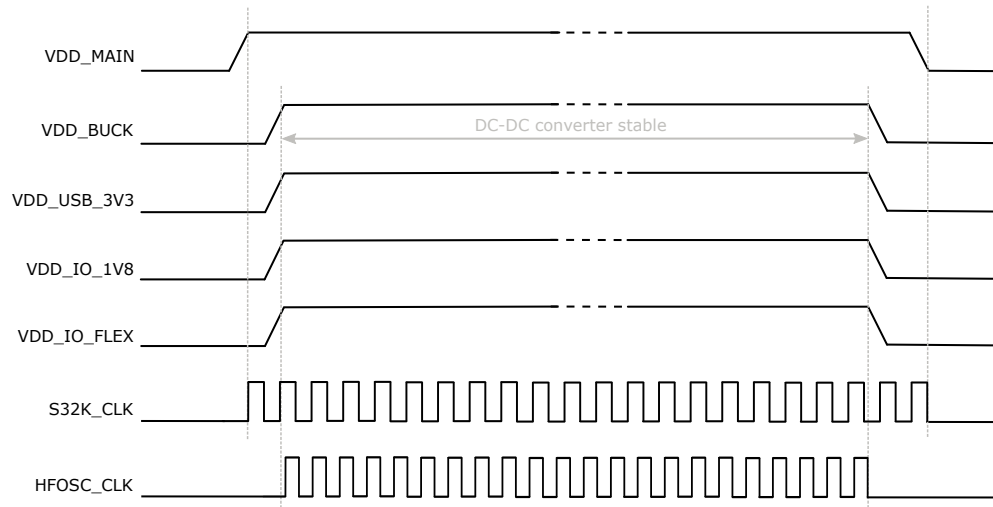
Figure 5-1 Power-Up/Power-Down Sequencing
