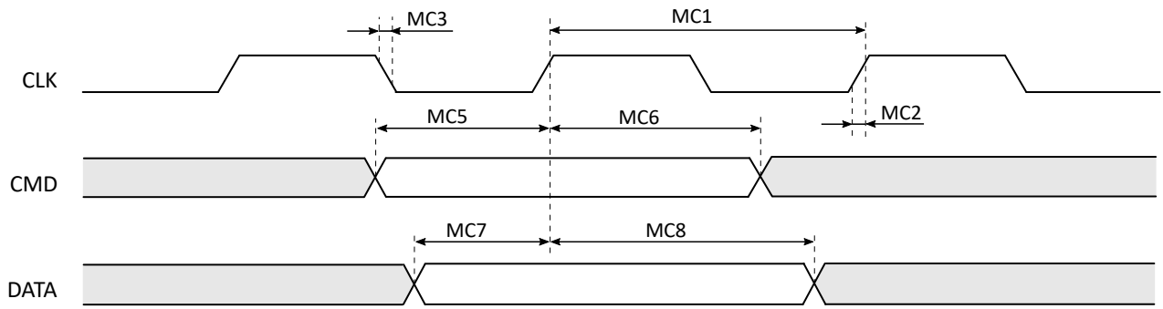
Figure 5-18 SDMMC Timing Diagram (SDR12/SDR25)
