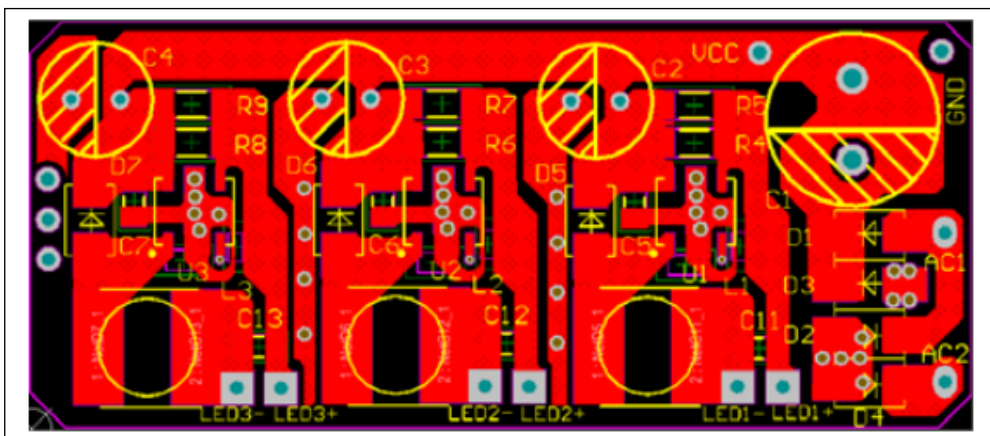
Figure 5 Board PCB Layout - Top Layer
