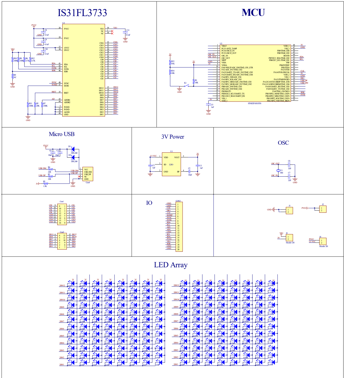
Figure 2 IS31FL3733 Application Schematic
