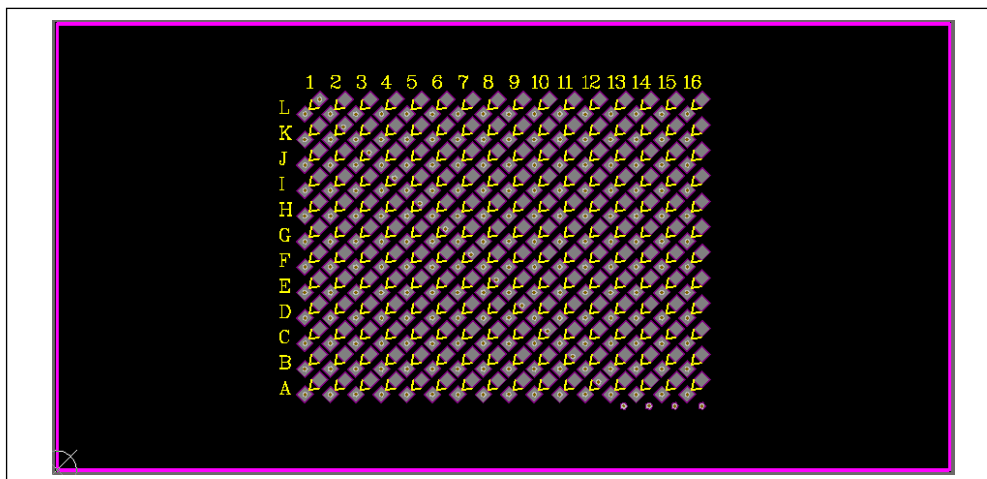
Figure 7 LED Board Component Placement Guide - Top Layer
