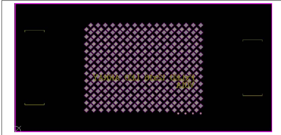
Figure 9 LED Board Component Placement Guide - Bottom Layer
