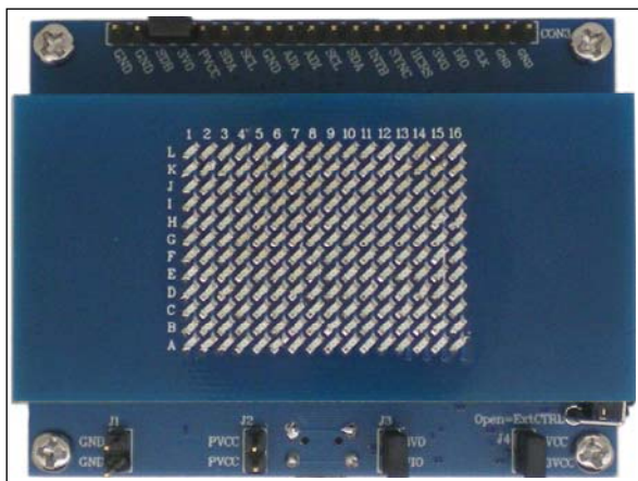
Figure 1 Photo of IS31FL3733 Evaluation Board
