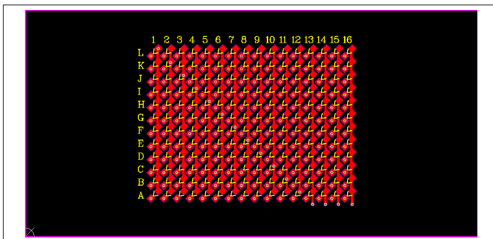
Figure 8 LED Board PCB Layout - Top Layer
