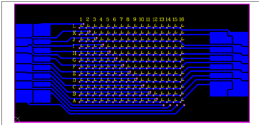
Figure 10 LED Board PCB Layout - Bottom Layer
