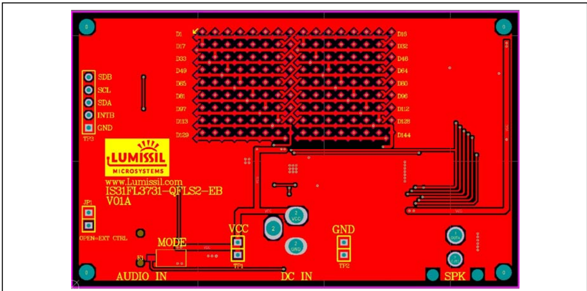
Figure 15 Board PCB Layout- Top Layer
