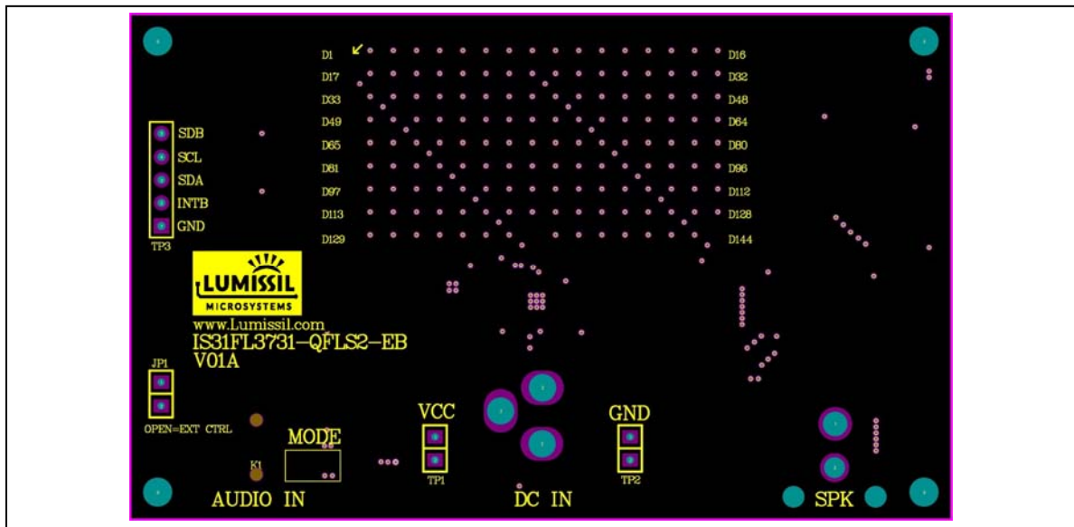
Figure 14 Board Component Placement Guide -Top Layer
