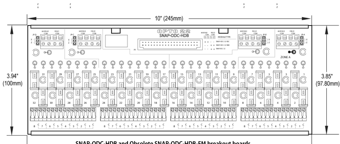
SNAP-ODC-HDB and Obsolete SNAP-ODC-HDB-FM breakout boards
