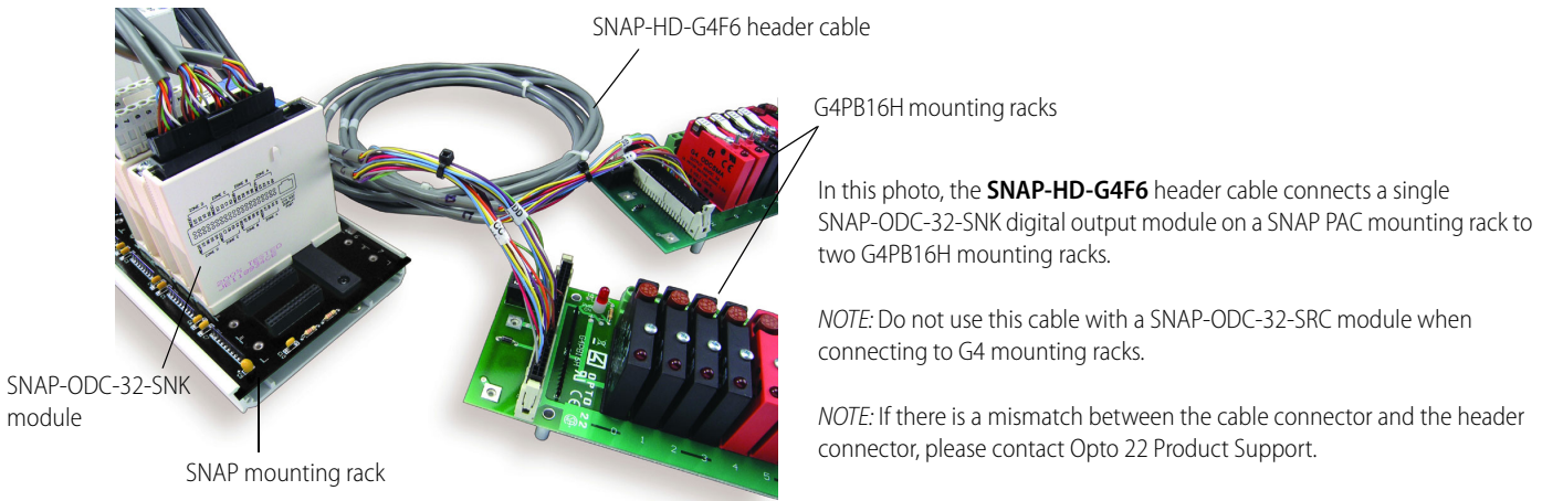
SNAP-HD-G4F6 cable
