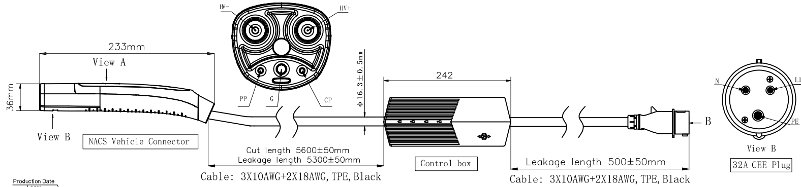
Vehicle Connector wiring diagram
