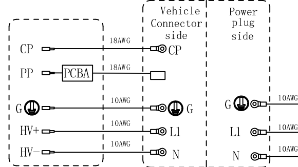
Vehicle Connector wiring diagram
