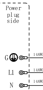
Control box wiring diagram
