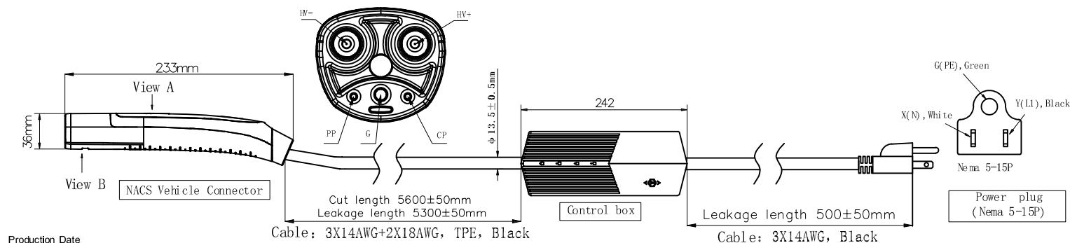
Vehicle Connector wiring diagram
