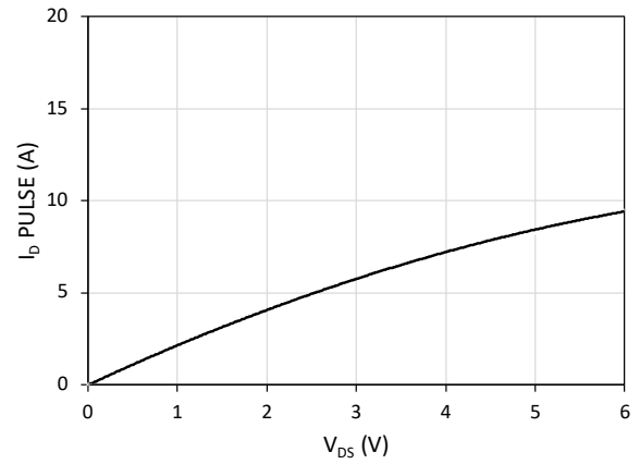
Figure 6. Pulsed Drain current ( I_D PULSE) vs. drain-to-source voltage ( V_{DS} ) at T = 125^\circ\text{C}
