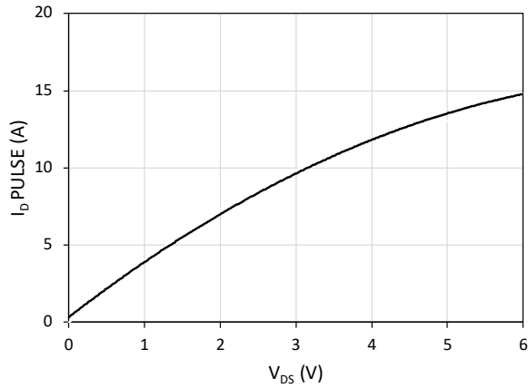
Figure 5. Pulsed Drain current ( I_D PULSE) vs. drain-to-source voltage ( V_{DS} ) at T = 25^\circ\text{C}
