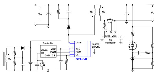
QR Flyback
