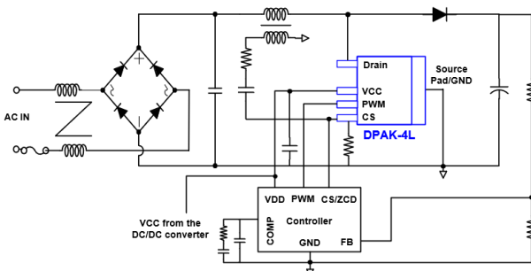
Boost PFC
