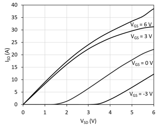
Fig. 4. Source-to-drain reverse conduction voltage at T = 150\text{ }^{\circ}\text{C}
