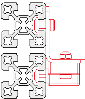
40 to 40 - Profile
