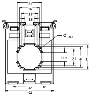
CT-500/5, 1000/5
