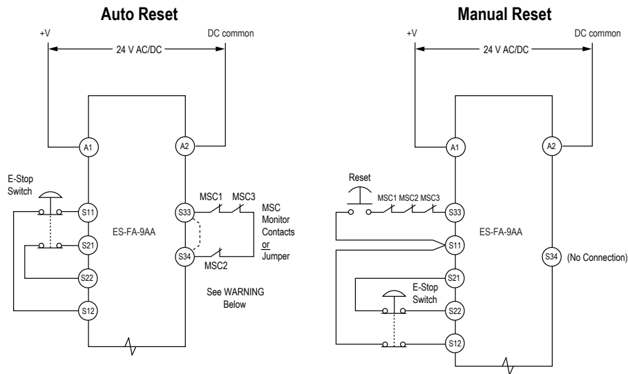
Dual-Channel E-Stop Applications
