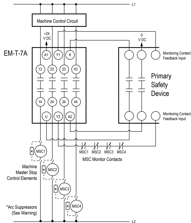
Generalized EM-T-7A Wiring for Two-Channel Control
