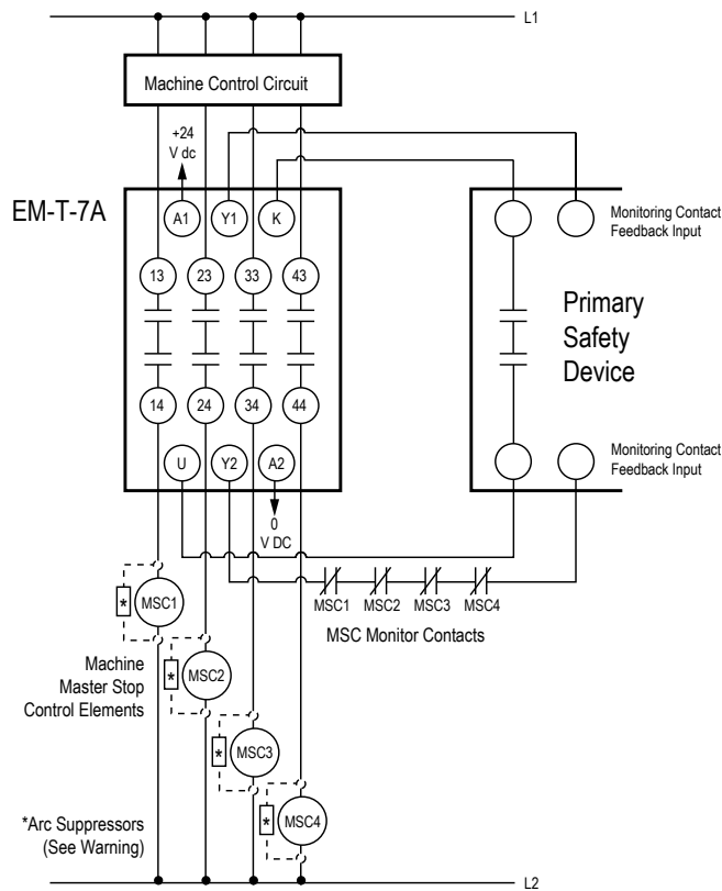
Generalized EM-T-7A Wiring for One-Channel Control
