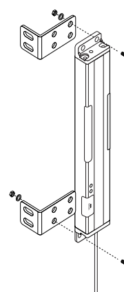
Mounting Hardware
