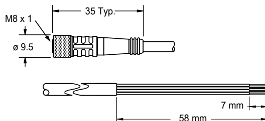
Female cordsets
