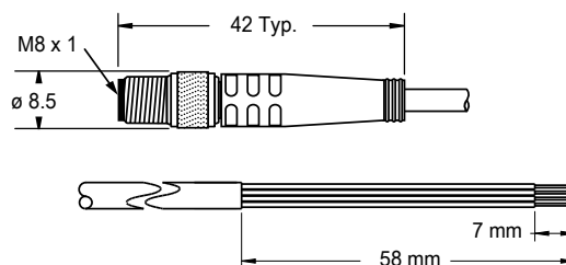
Male cordsets
