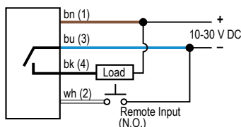
NPN and Remote Input
