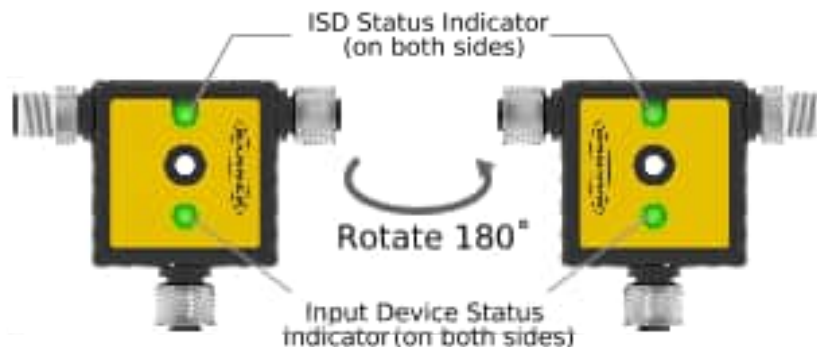
Figure 11. SSA-ISD Connect status indicators
