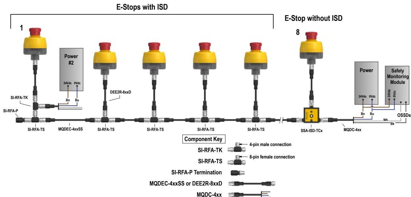
Figure 6. Option 1: Use a SI-RFA-TK Reset Connector in series with ISD Device. If available, set the power supplies for parallel output.
