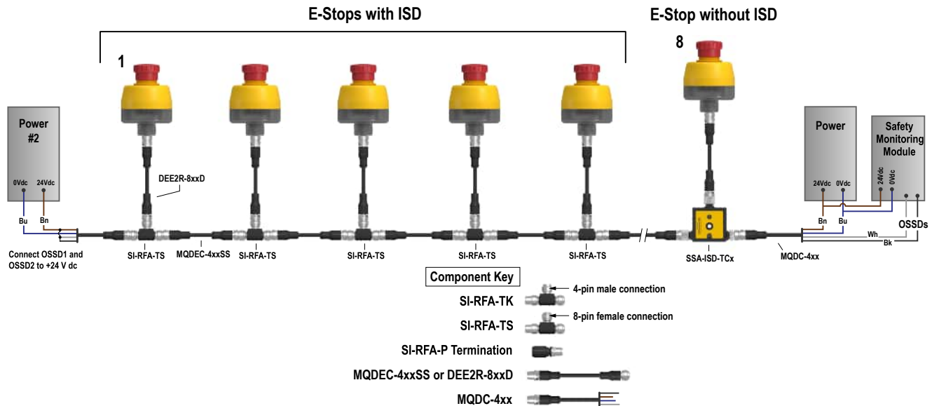
Figure 7. Option 2: Replace the terminator with a power supply. The OSSD1 and OSSD2 wires at power supply #2 must be connected to +24 V DC. If available, set the power supplies for parallel output.
