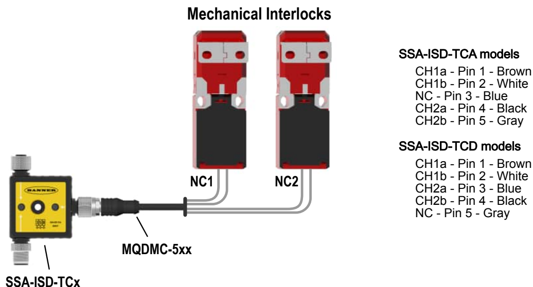
Figure 3. Wiring the SSA-ISD Connect to mechanical interlocks
