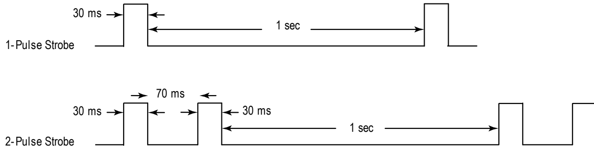
Timing diagram for 1 pulse or 2 pulses
