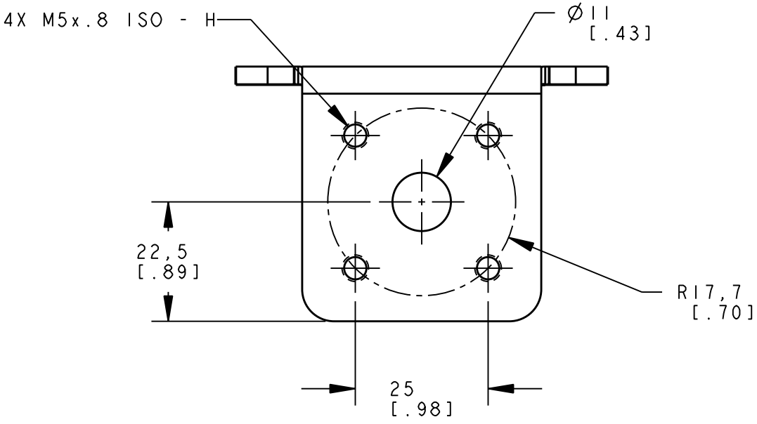
VIEW Z-Z
