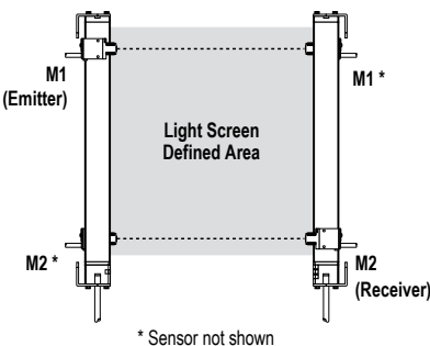
Figure 37. Horizontal photoelectric muting devices placed at different heights
