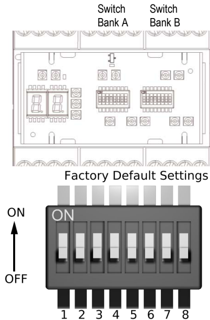
Figure 4. Muting Module manual configuration parameters
