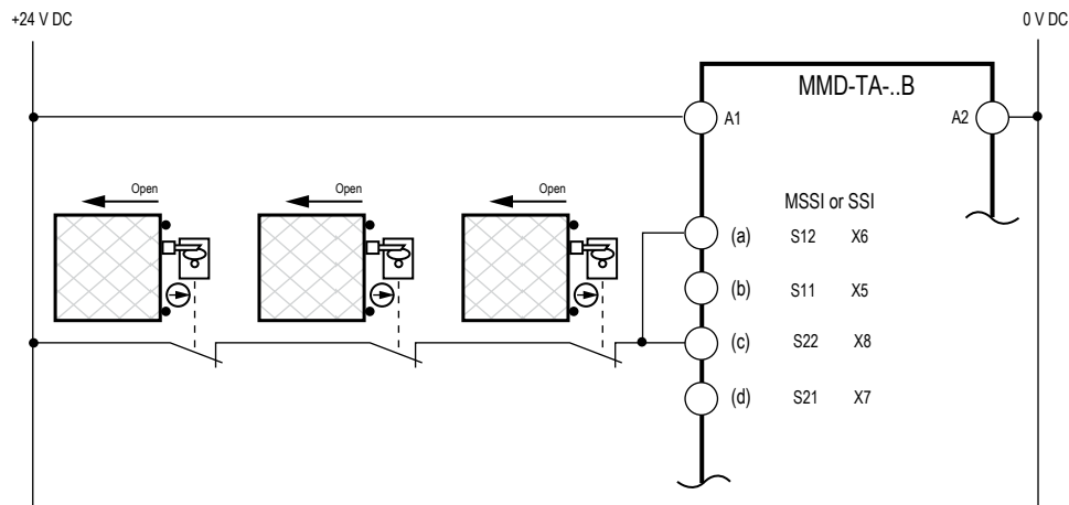
Figure 26. MSSl or SSl Category 2 interfacing: positive opening
