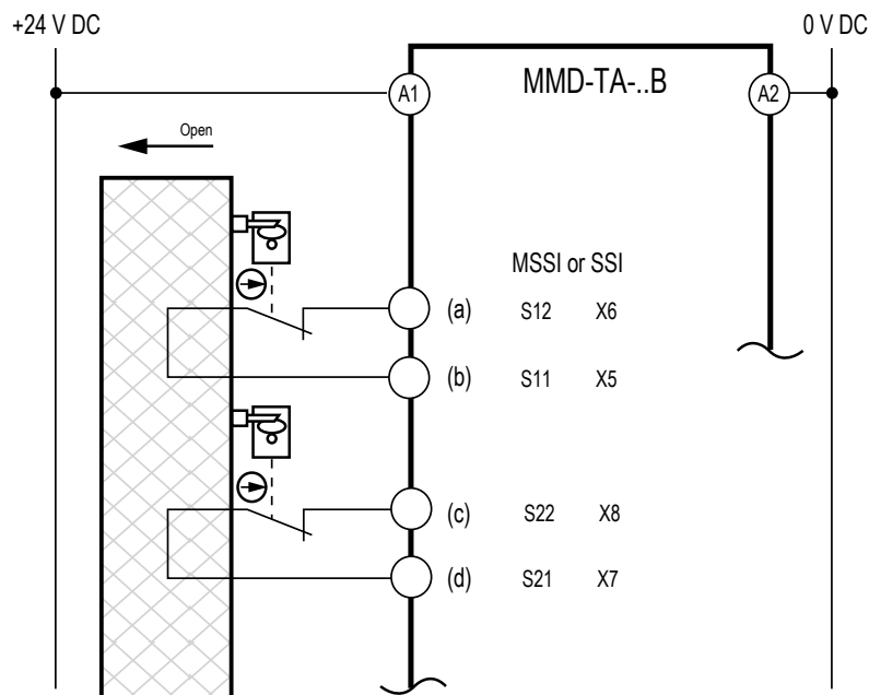
Figure 28. SSl Category 4 interfacing: positive-opening interlocking switch(es)
