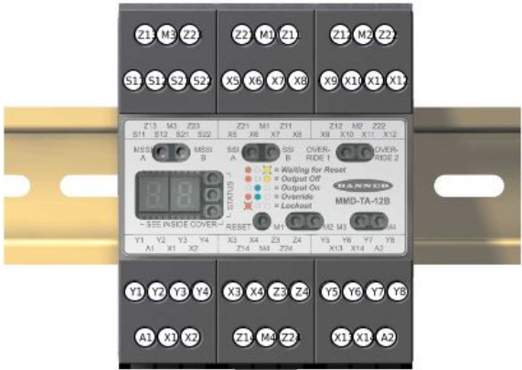
Figure 6. MMD-TA-12B terminal connection locations
