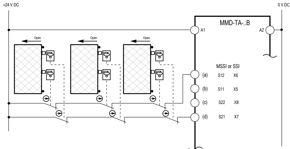
Figure 27. MSSl or SSl Category 3 interfacing: Positive-opening Interlocking switch(es)
